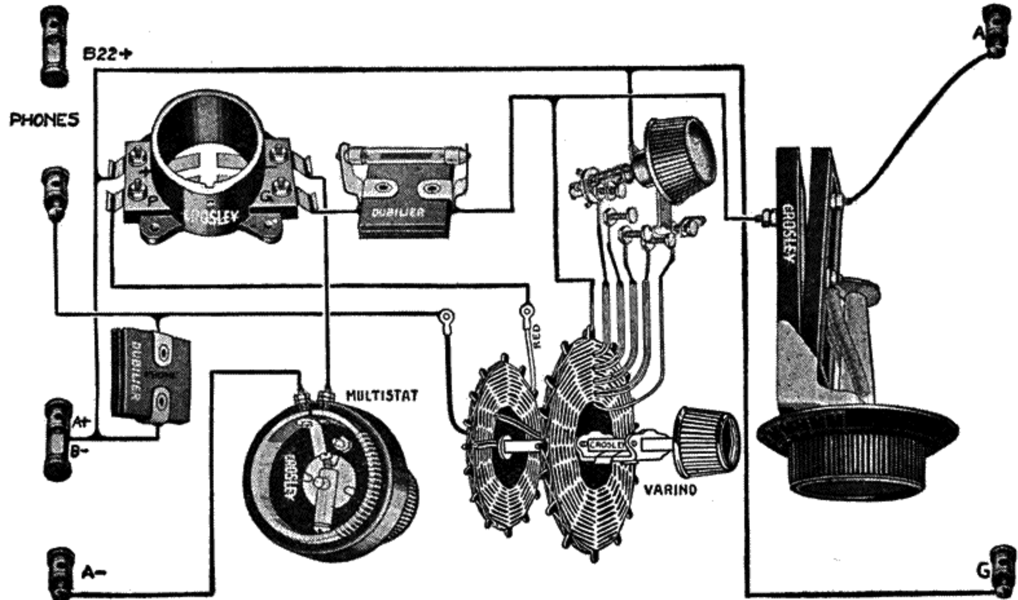
Crosley Type V Single Tube Regenerative Receiver
