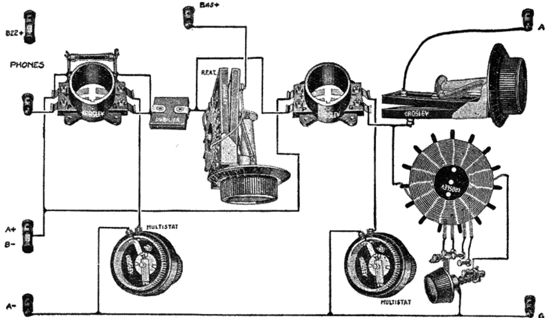
Crosley Model VI Circuit
