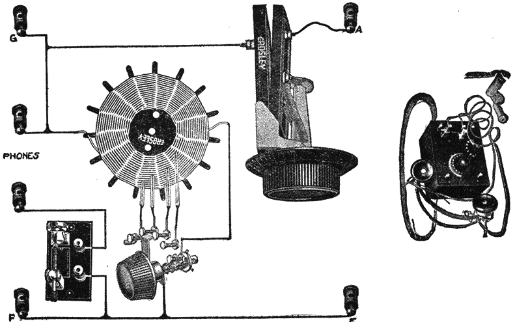
Crosley Crystal Receiver
